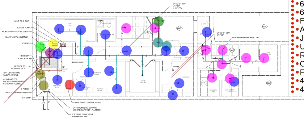
1 PROPOSED PLAN - CELLAR
