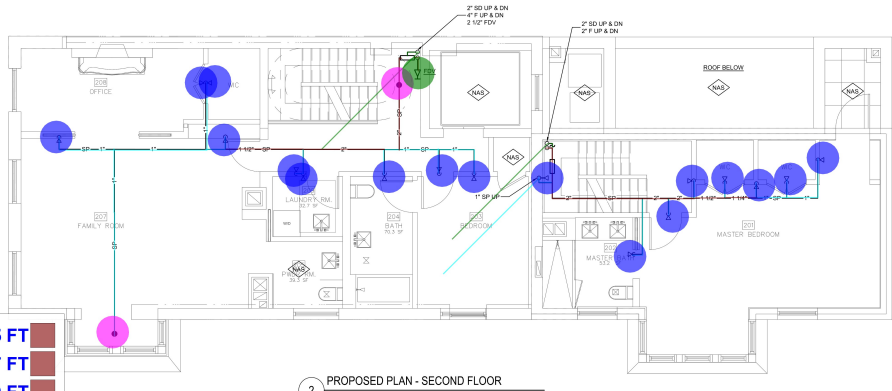
2 PROPOSED PLAN - SECOND FLOOR
