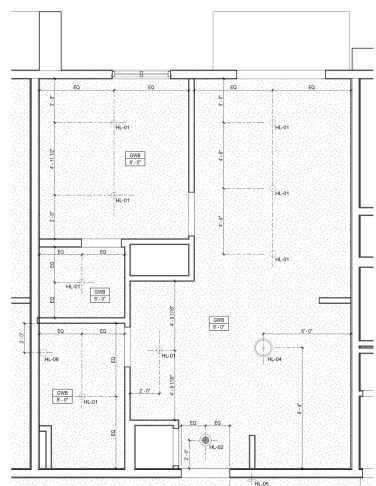
1 ENLARGED GUEST ROOM RCP - SUITE 1B A2.1B SCALE 3/8" = 1'-0"
