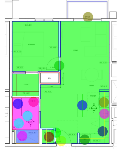
1 ENLARGED GUEST ROOM PLAN - SUITE 1B A2.1B SCALE 3/8" = 1'-0"
