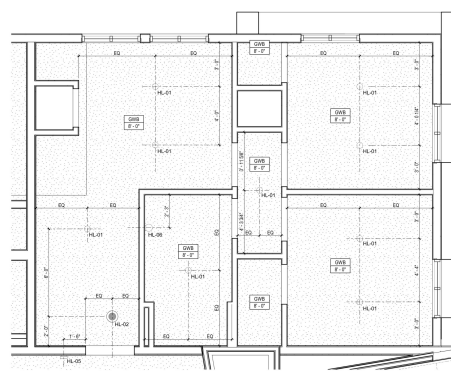
7 ENLARGED GUEST ROOM RCP - SUITE 2A A2.2A SCALE: 3/8"=1'-0"
