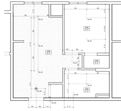
ENLARGED GUEST ROOM RCP - SUITE 1A SCALE: 1/4" = 1'-0"
