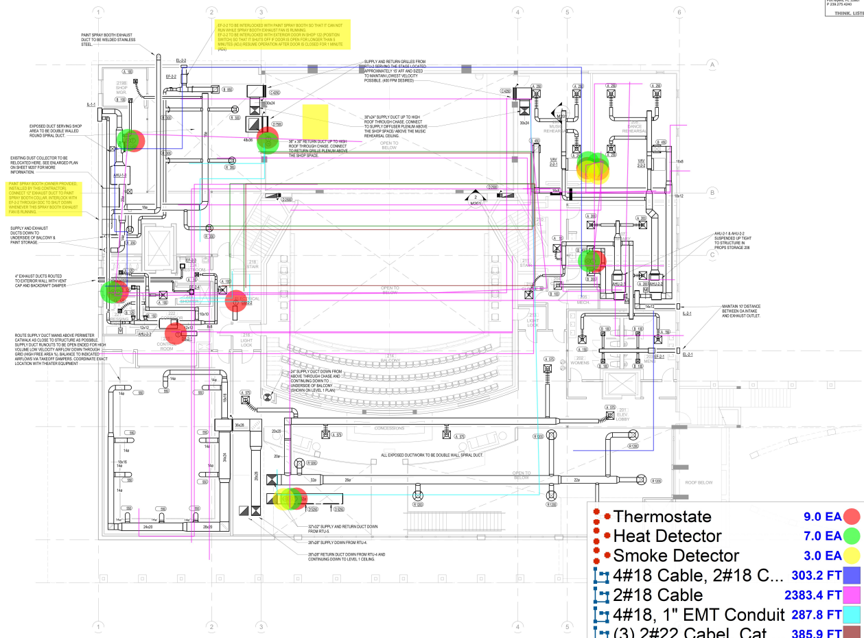
1 SECOND FLOOR PLAN - HVAC NEW CONSTRUCTION 1/8" = 1'-0"
